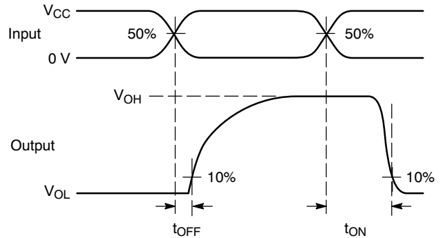
Figure 9. t_{ON}/t_{OFF}
